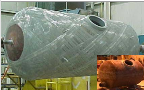
S Series Dual Construction Method: Shell & Winding
